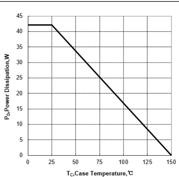
Figure 2c Power Dissipation (TO-220F)
